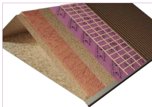
SIPS Warm Roof Construction
